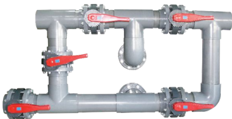
5 Way Butterfly Valve NBV30-NBV80
