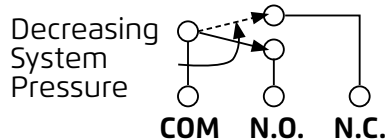
Typical Low Pressure Supervision
